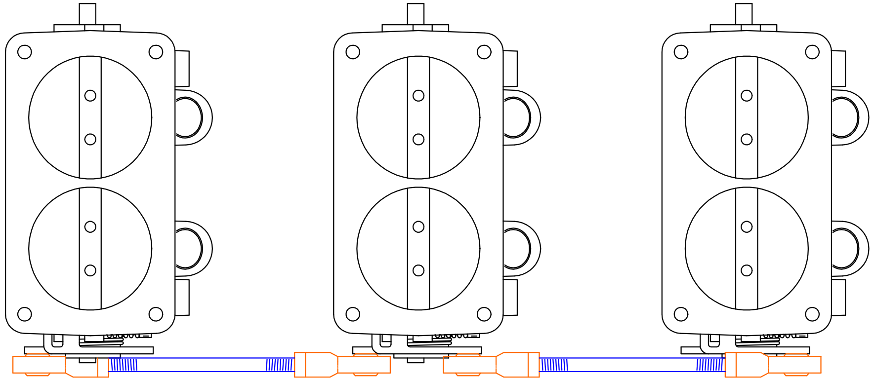
Typical linkage. TC throttle bodies
