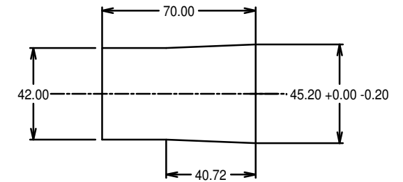
Bore Profile - circular section
