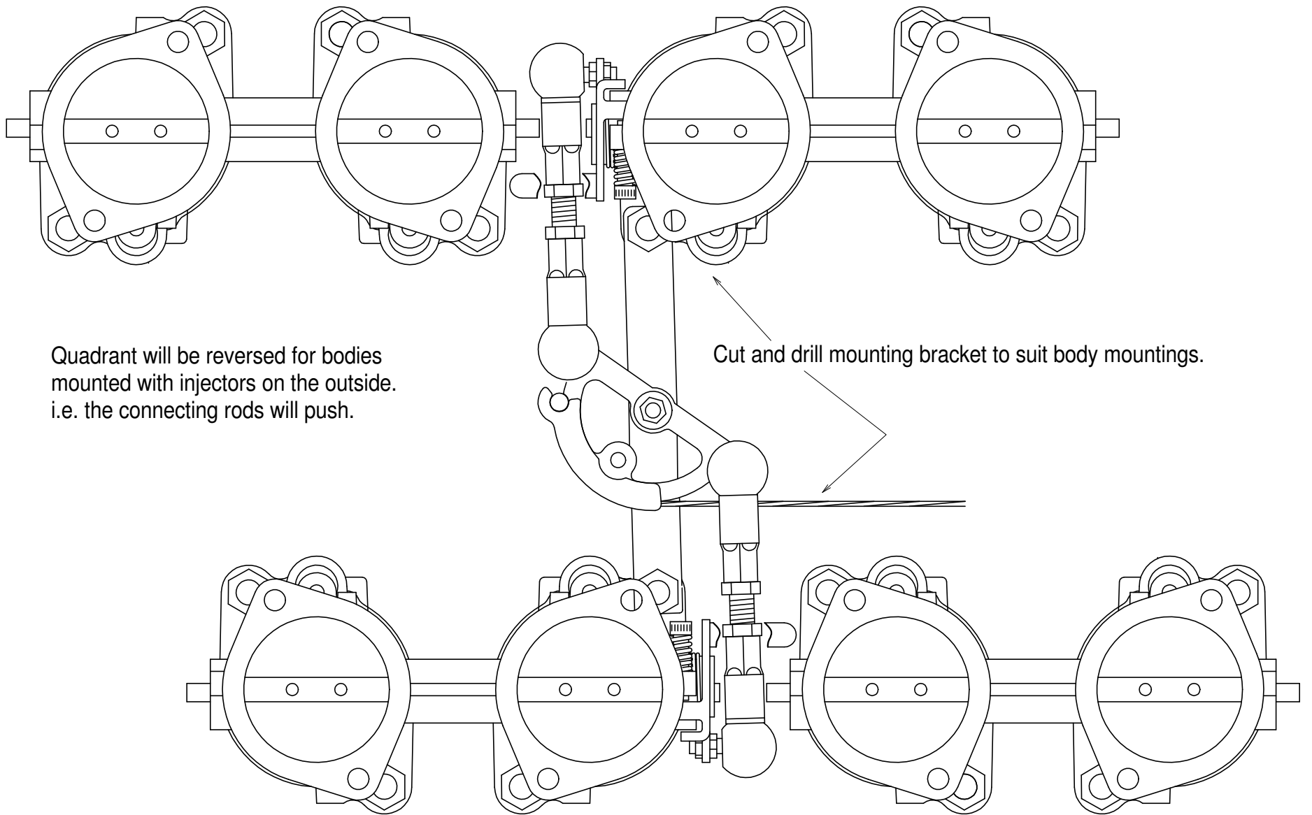
'V' engine linkage. Typical layout.
